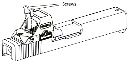
Fig. 5 Mounting on the slide
